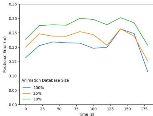
Figure 7: Positional error (distance between the user and the avatar) for different animation database sizes using the same user input. 100% is our complete animation database, while the others contain 25% and 10% of the poses in the complete database. The error is averaged every 20 seconds. Large databases represent a wider range of motions and better match the user's trajectories, thus minimizing the positional error.
